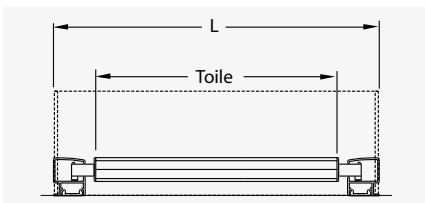
Guidage coulisses
