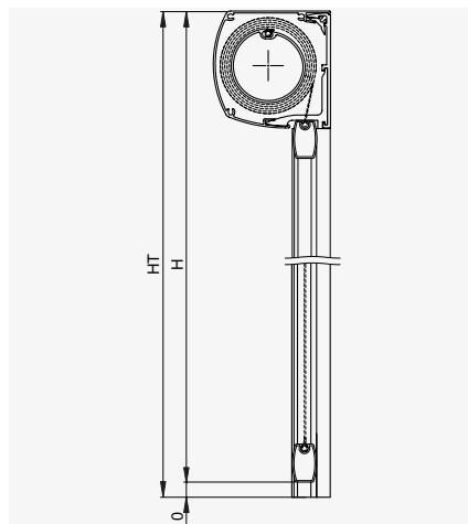
Guidage coulisses
